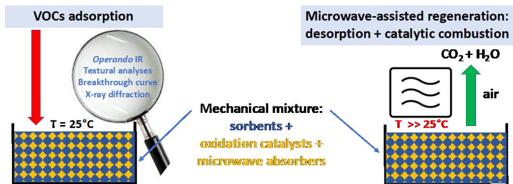
Figure 1. Schematic representation of the project: use various advanced characterization methods to understand VOCs adsorptions in sorbents and the ex situ regeneration in a common microwave oven. The system will consist of sorbents mixed with oxidation catalysts exhibiting high dielectric constants.
